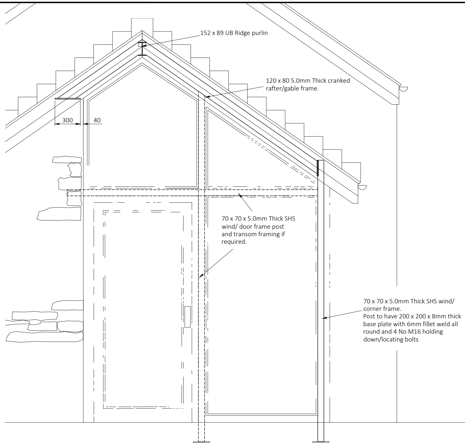
Entrance - North Elevation (Showing Extension Steelwork) (1:25)
