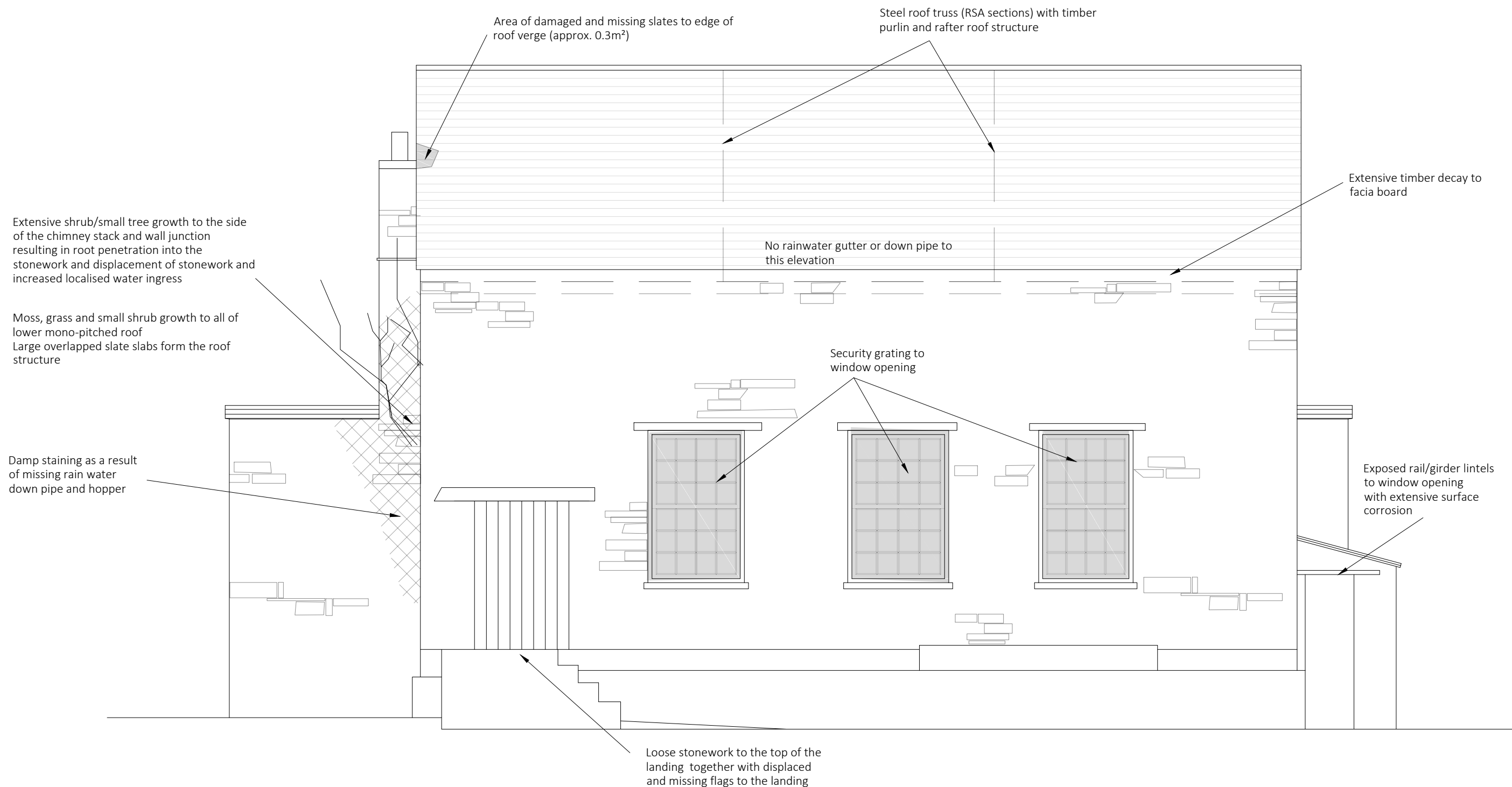
Elevation B - West (Showing defects and areas of further investigation require) (1:50)
