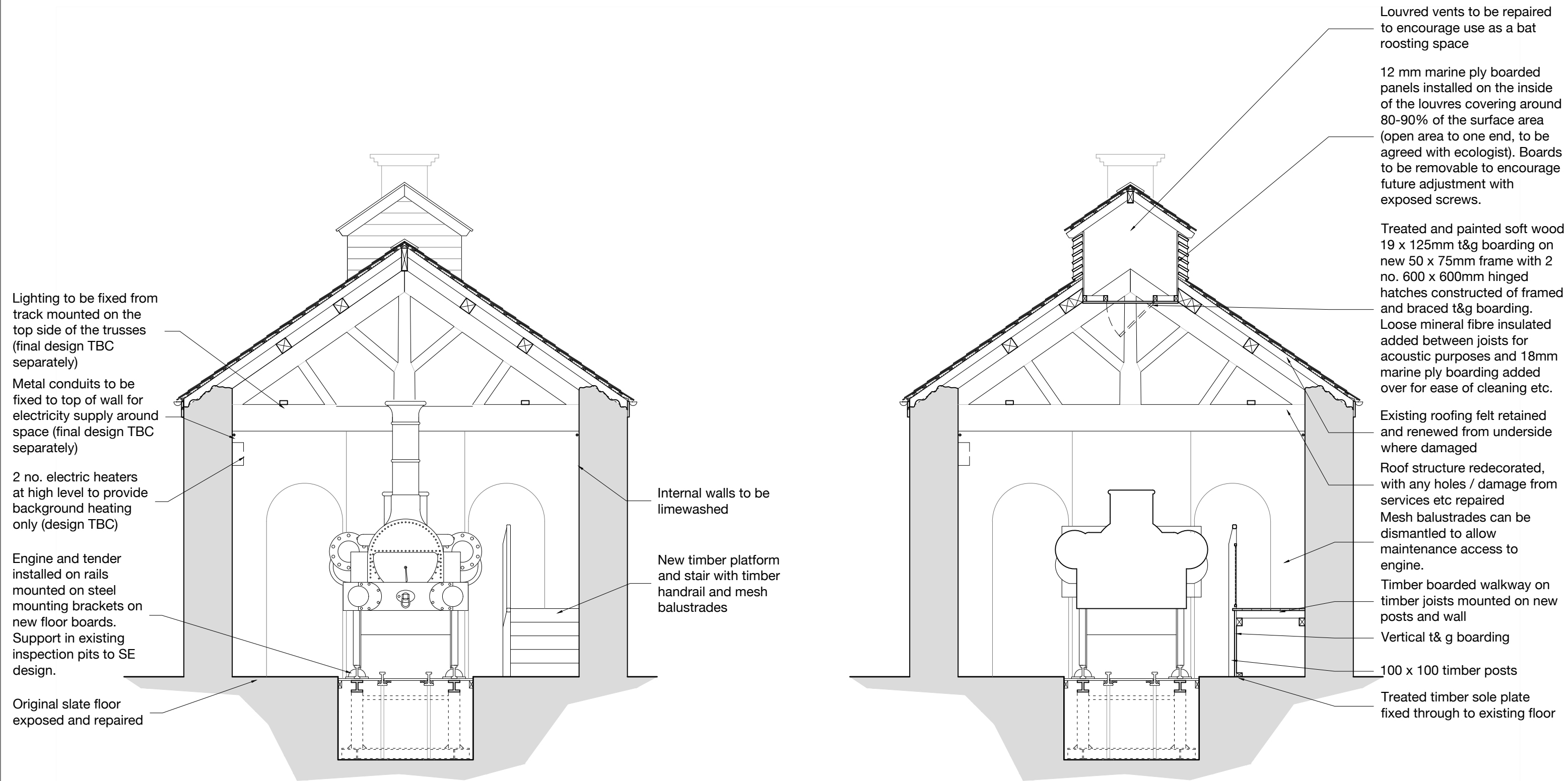
Section BB - Cross Section as Proposed (1:50 at A3)
