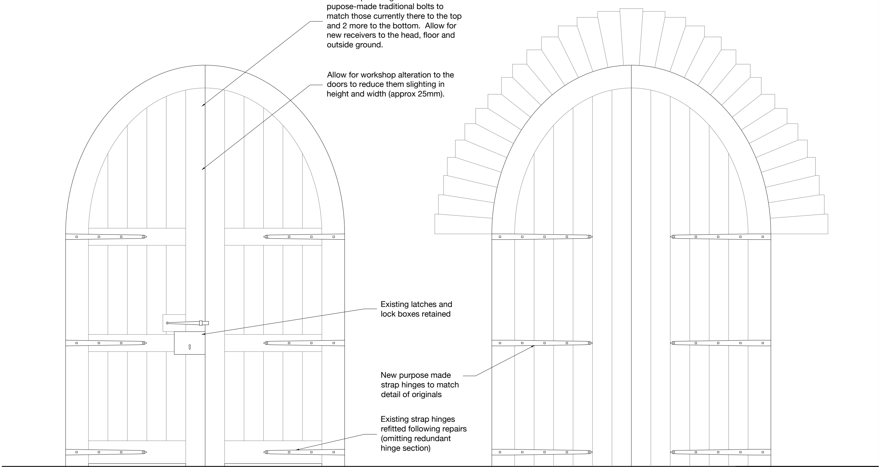
Inside Face of Timber Door (Sitting on the Outside of New Glazed Door - not Shown) (1:20 at A3)
