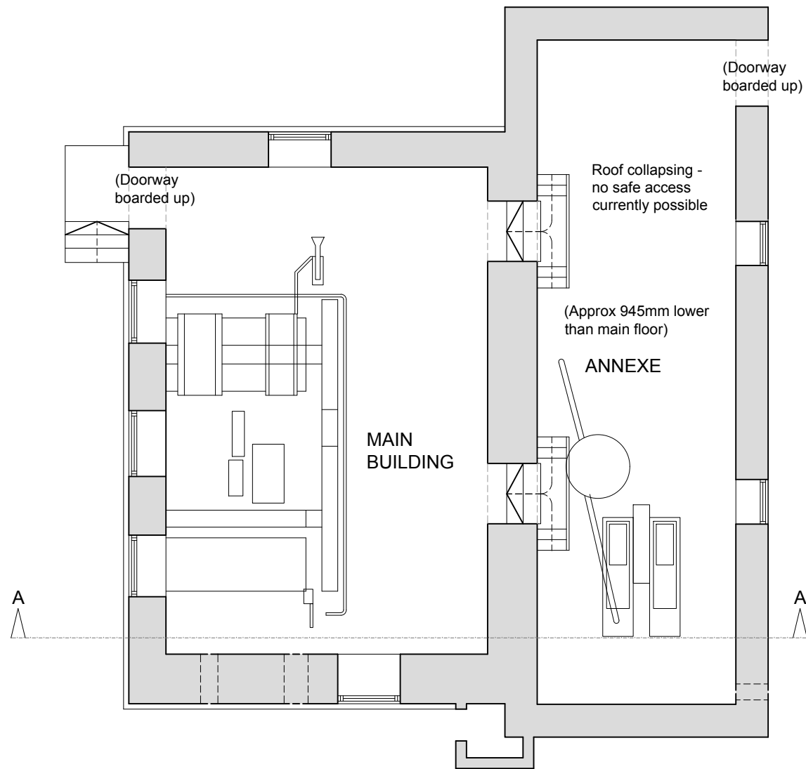
Plan as Existing (1:100 at A3)
