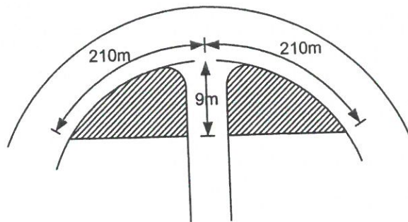
Junction Type 1 Detail 1
