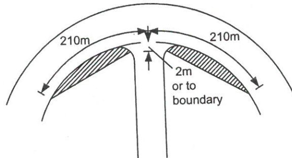
Junction Type 3 Detail 3
