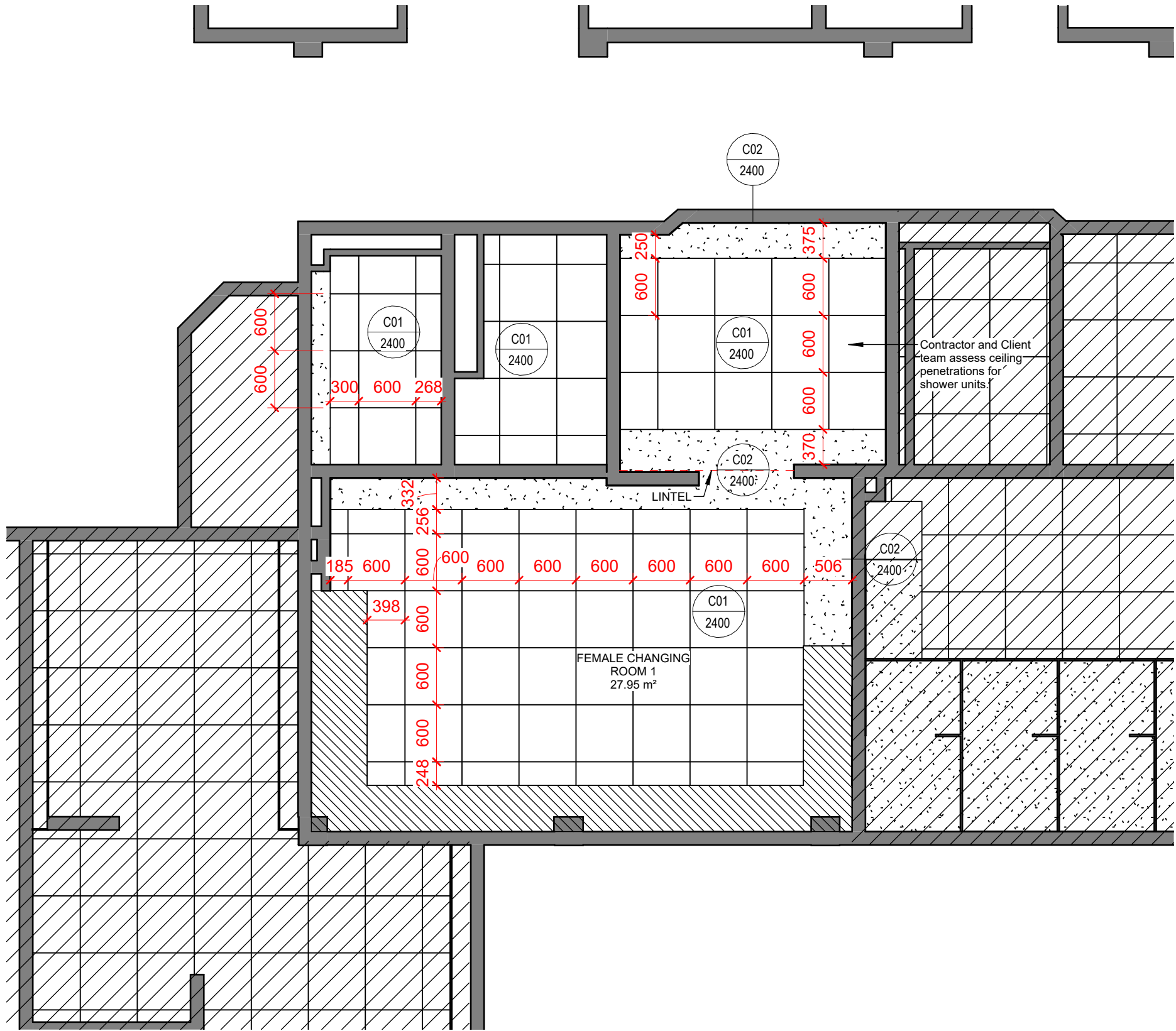
Reflected Ceiling Plan - Female Changing Room 1 : 50
