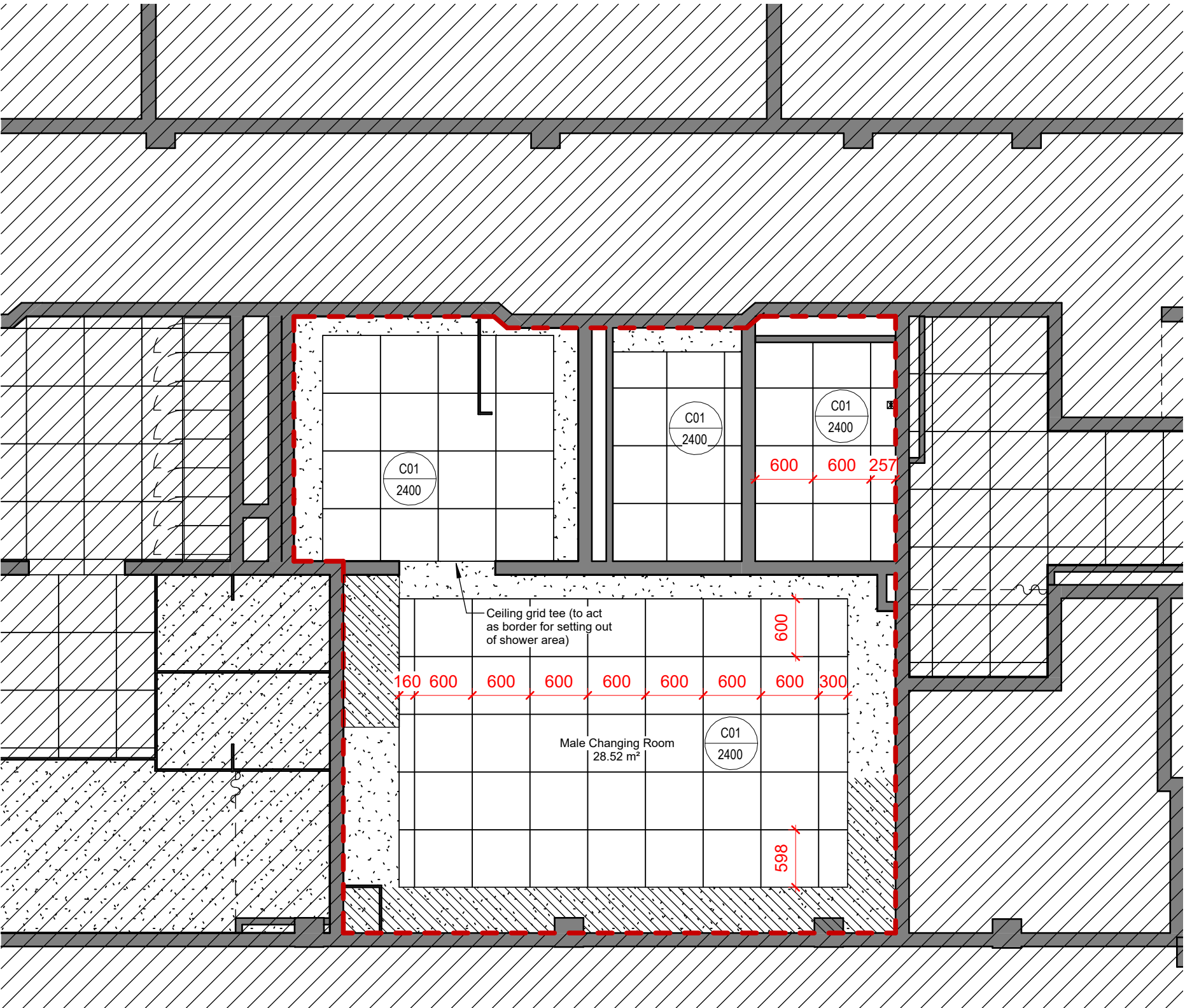
Reflected Ceiling Plan - Male Changing Room 1 : 50
