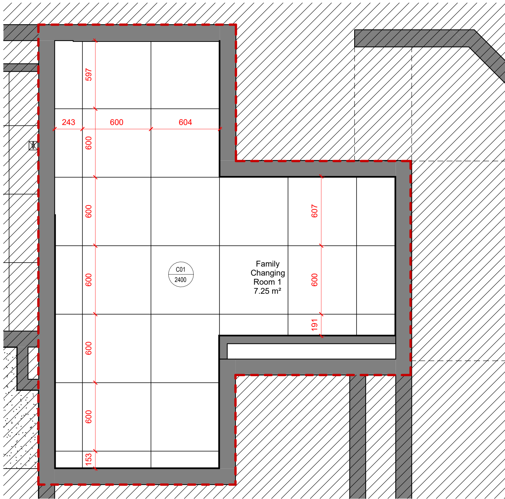
Reflected Ceiling Plan - Family Changing Room 1 1 : 20
