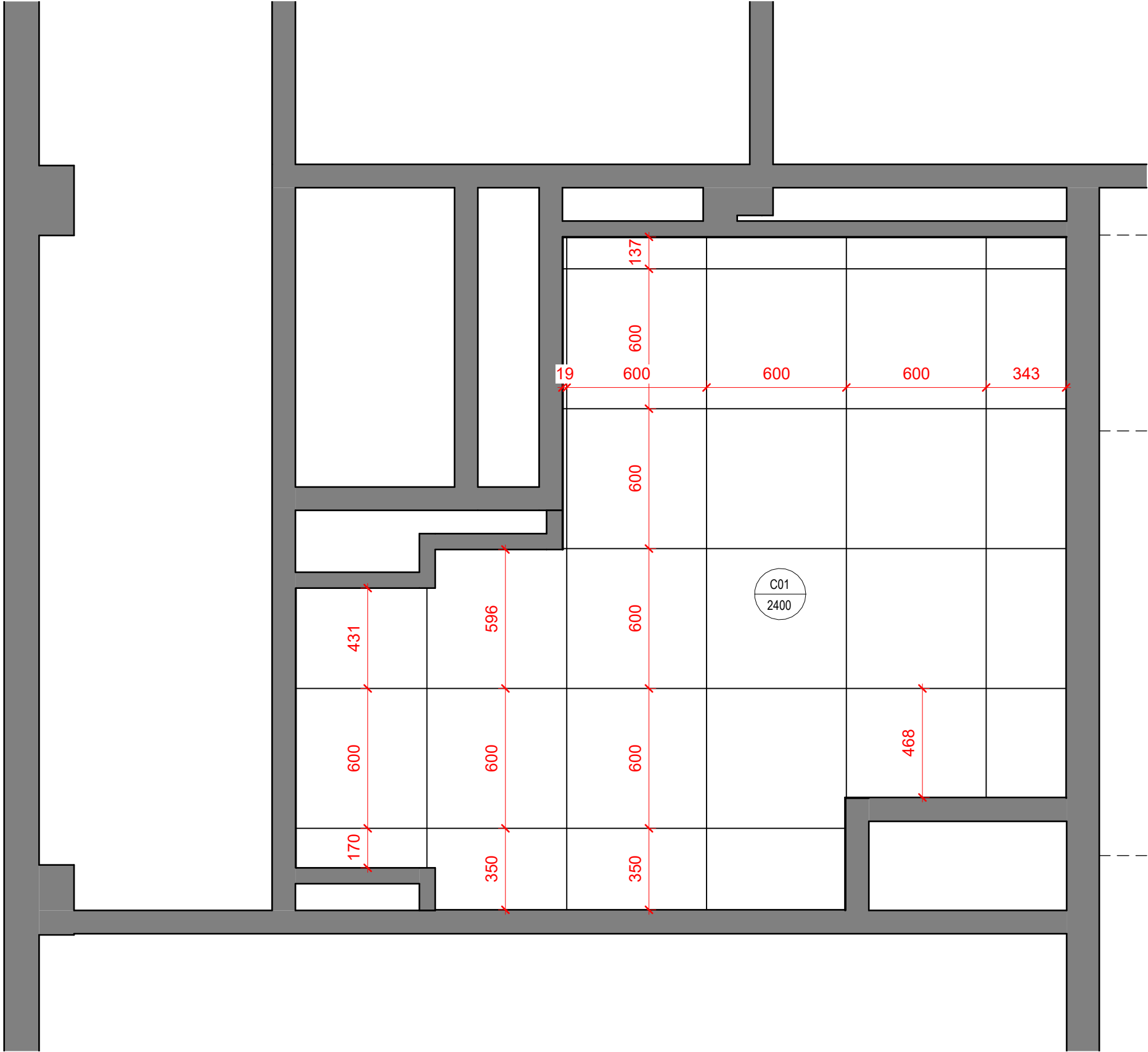
Reflected Ceiling Plan - Family Changing Room 2 1 : 20
