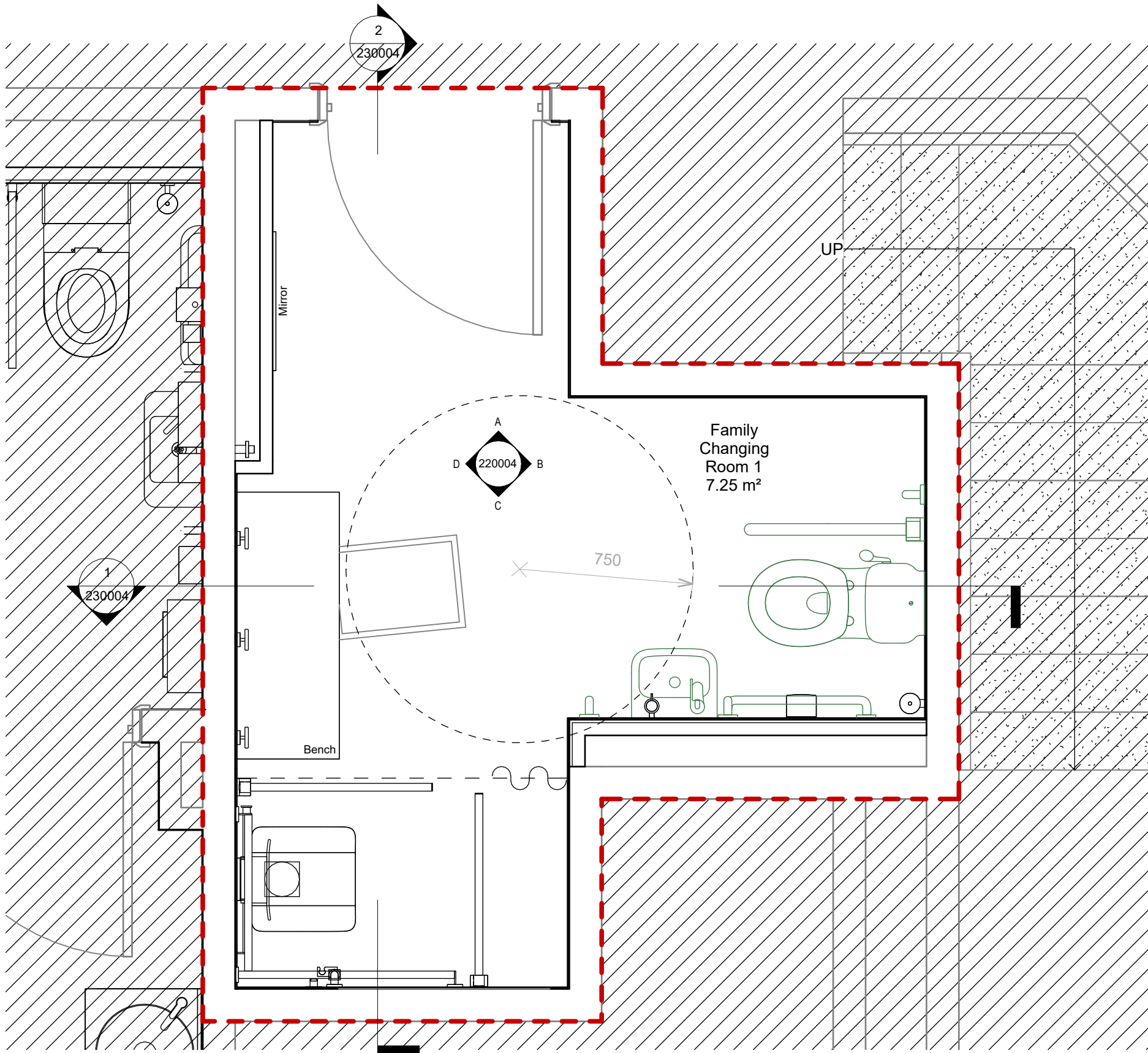
Proposed Family Changing Room 1 1 : 20
