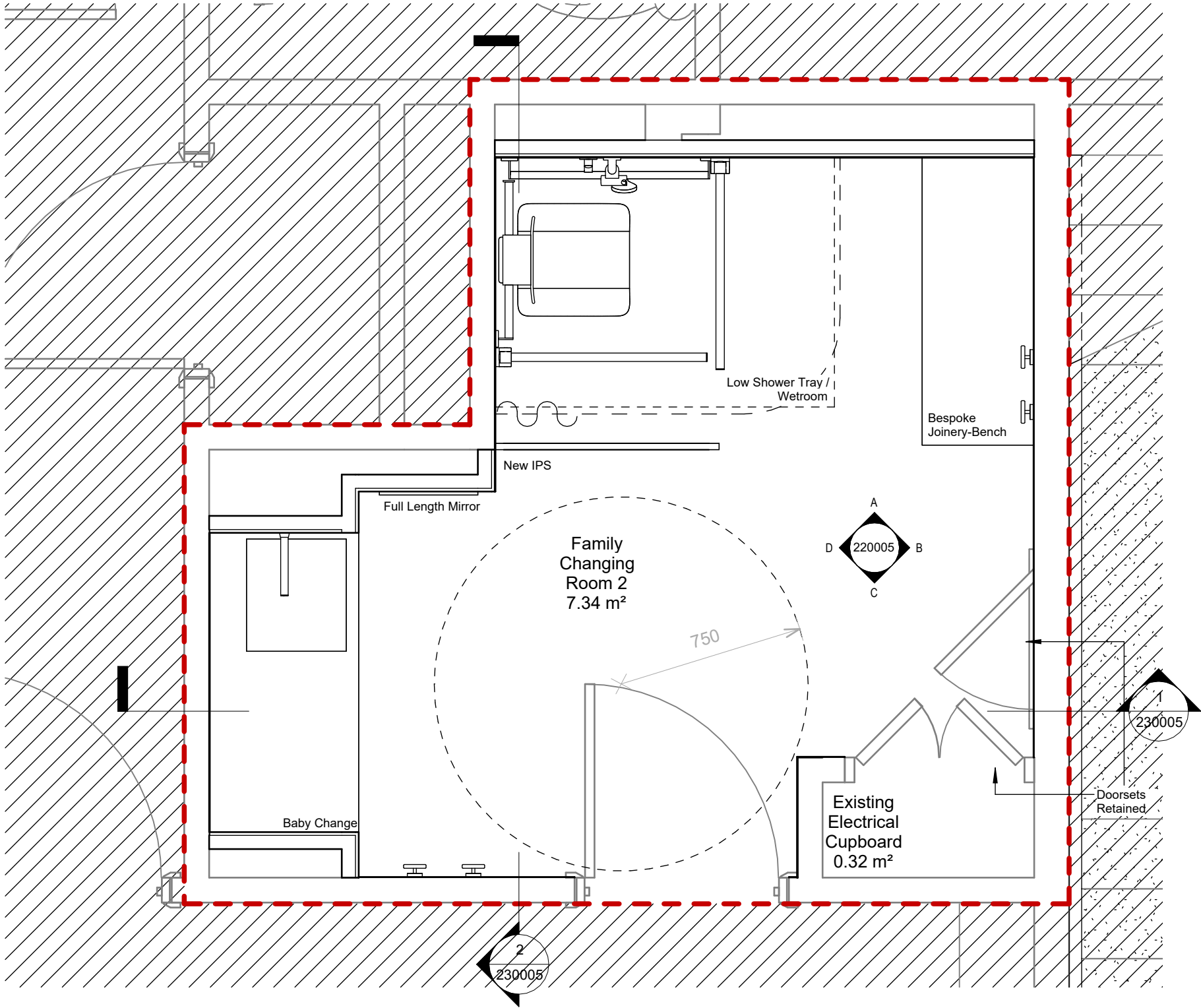
Proposed Family Changing Room 2 1 : 20
