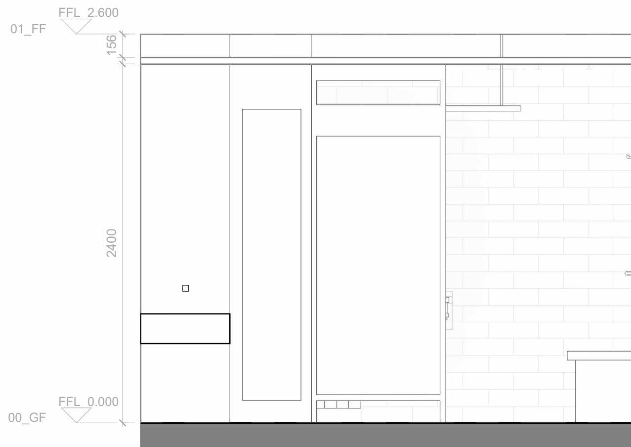
Family Changing Room 2 Section 1 1 : 25
