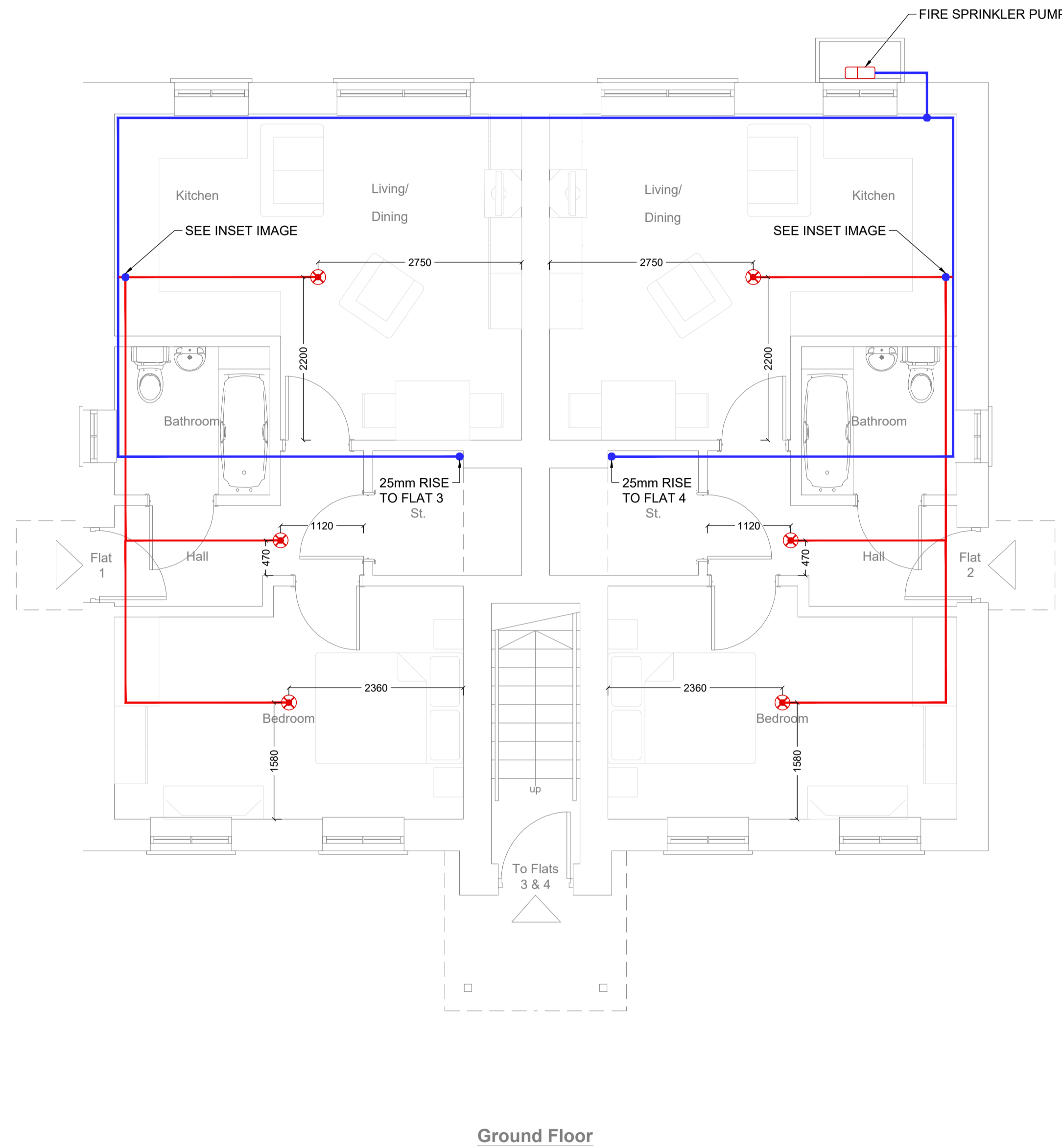
Ground Floor
